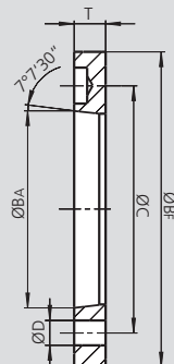
Type FF 1 ISO-A direct mounting
