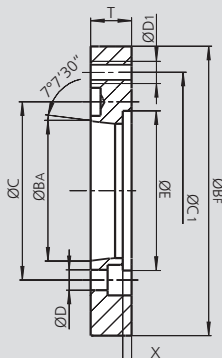
Type FF 2 ISO-A reduced mounting
