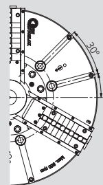
Ø 800 - 3 jaw
