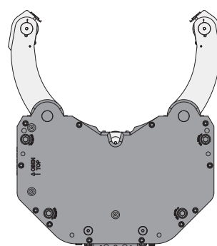
RX 6 Clamping range 100 - 520 mm
